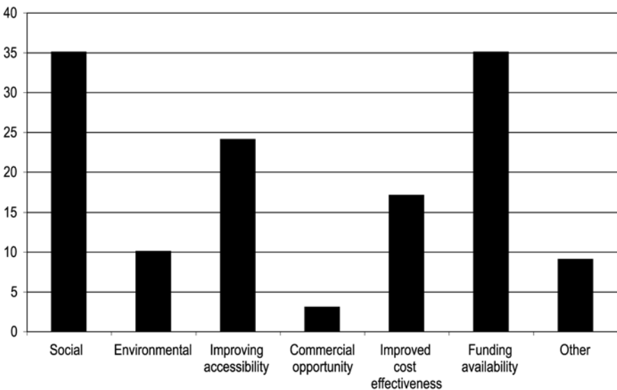
Figure 3. Scheme Catalysts
